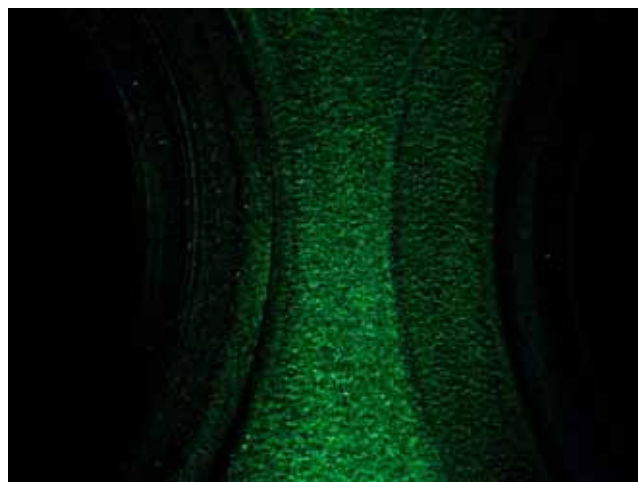
Between valve seat not found crack.
