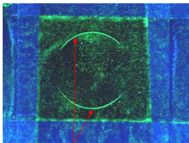
Test piece found crack.
